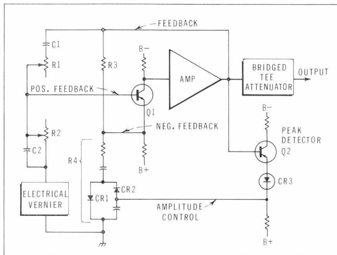
Fig. 3. Basic circuit arrangement of new RC oscillator. For power economy new amplitude control circuit replaces traditional ballast lamp, but frequency response is very constant as shown in Fig. 5.
